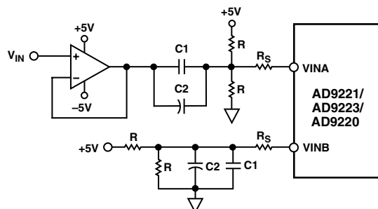
Figure 16. AC-Coupled Input-Flexible Input Span, V CM = 2 V
