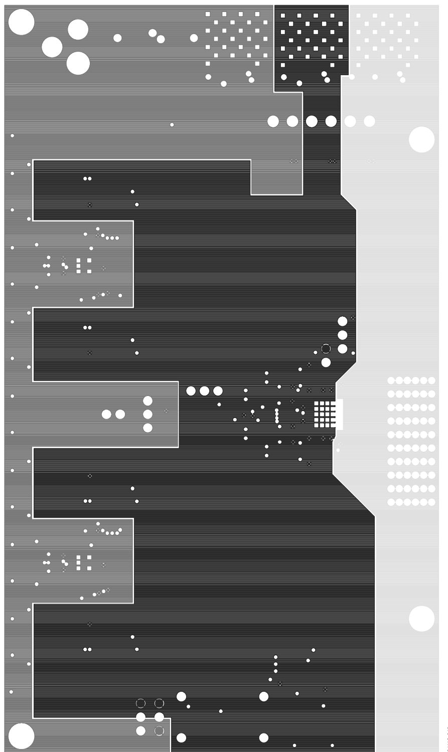
Figure 56. Evaluation Board Layout, Power Plane
