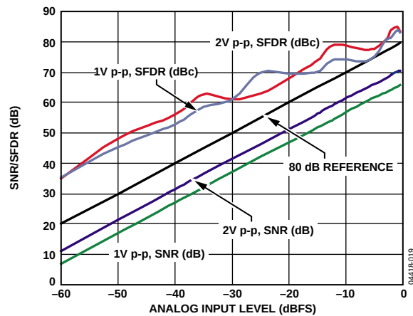
Figure 19. SNR/SFDR vs. Analog Input Level, f_{\text{IN}} = 10.3 \text{ MHz} , f_{\text{SAMPLE}} = 65 \text{ MSPS}
