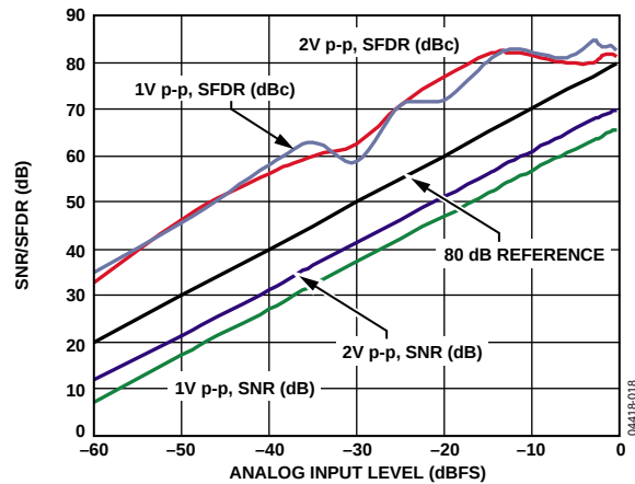
Figure 18. SNR/SFDR vs. Analog Input Level, f_{\text{IN}} = 25 \text{ MHz} , f_{\text{SAMPLE}} = 50 \text{ MSPS}
