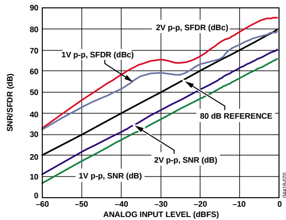
Figure 20. SNR/SFDR vs. Analog Input Level, f_{\text{IN}} = 30 \text{ MHz} , f_{\text{SAMPLE}} = 65 \text{ MSPS}
