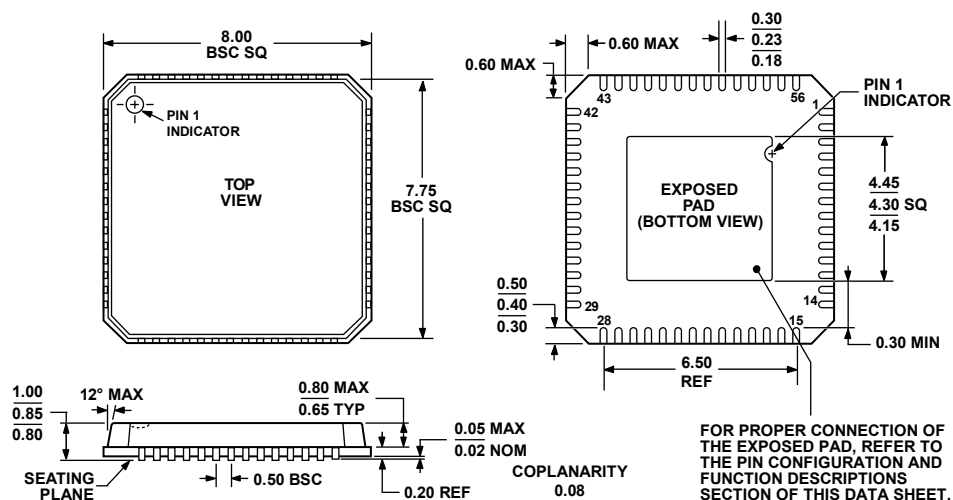
Figure 34. 56-Lead Lead Frame Chip Scale Package [LFCSP_VQ]
