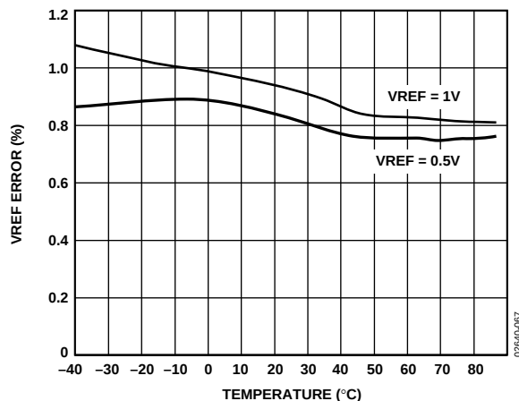
Figure 37. Typical VREF Drift
