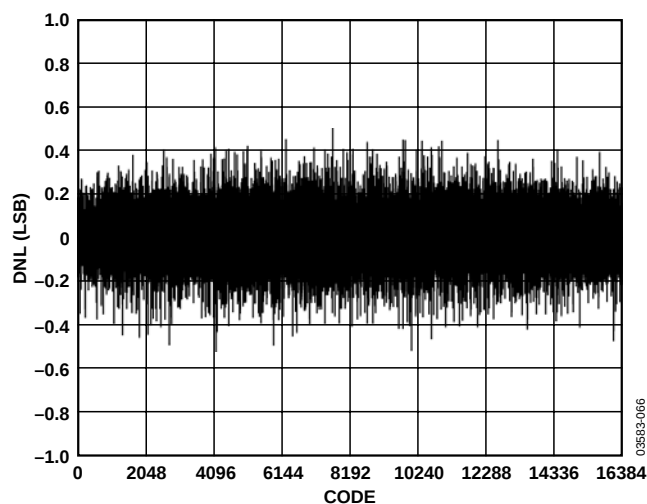
Figure 30. AD9245-65 Typical DNL
