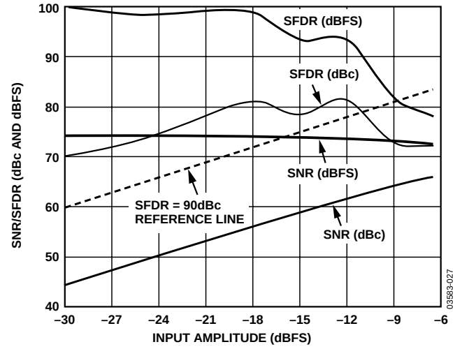
Figure 18. Two-Tone SNR/SFDR vs. Input Amplitude @ 69 MHz and 70 MHz
