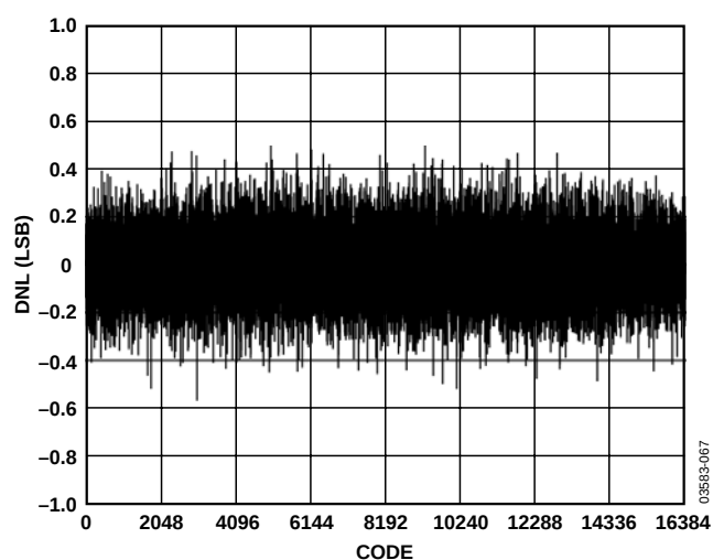
Figure 31. AD9245-40 Typical DNL
