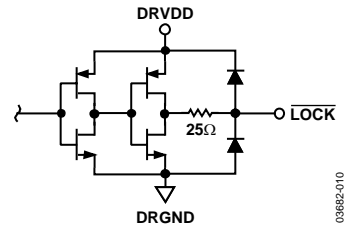
Figure 8. Equivalent LOCK Output Circuit
