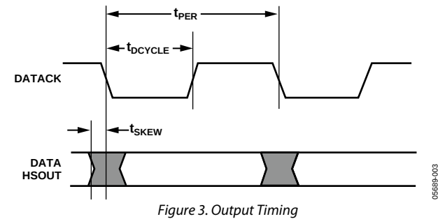
Figure 3. Output Timing
