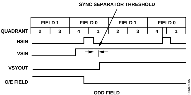
Figure 5. VSYNC Filter—Odd/Even
