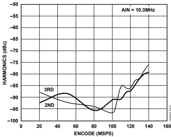
Figure 6. Second-Order and Third-Order Harmonics vs. f_s , f_{IN} = 10.3 MHz
