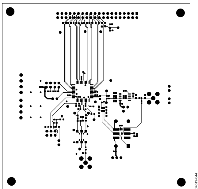
Figure 44. PCB Top-Side Copper Routing
