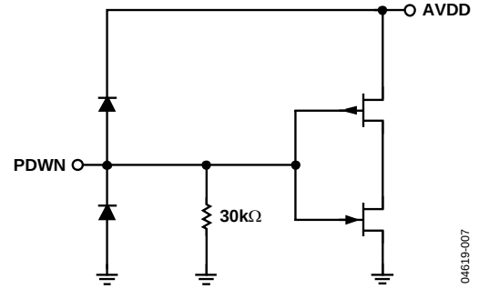
Figure 27. Power-Down Input
