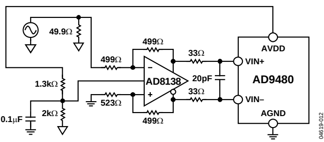
Figure 32. Driving the ADC with the AD8138
