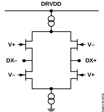
Figure 29. LVDS Data, DCO Outputs
