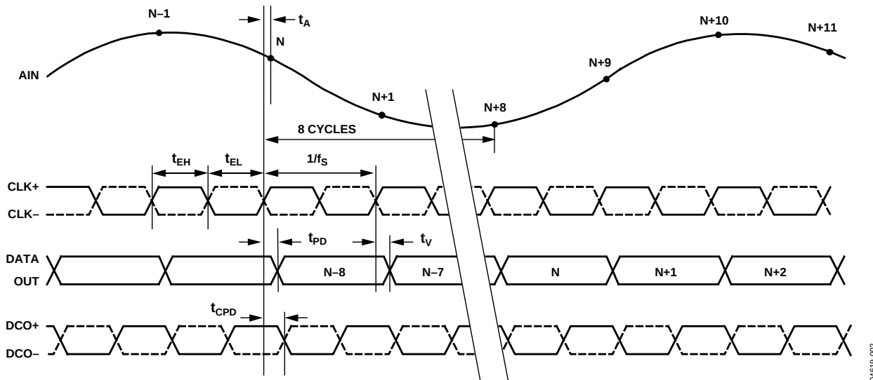
Figure 2. Timing Diagram
