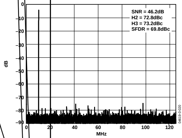
Figure 20. FFT: f_s = 250 \text{ MSPS} , A_{IN} = 10.3 \text{ MHz @ } -1 \text{ dBFS}
