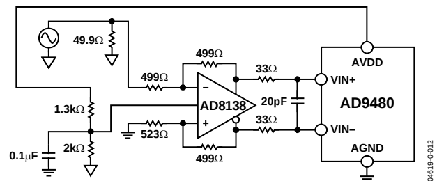
Figure 12. Driving the ADC with the AD8138
