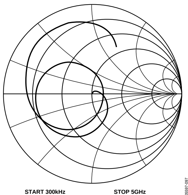
Figure 9. CLK Smith Chart (Evaluation Board)
