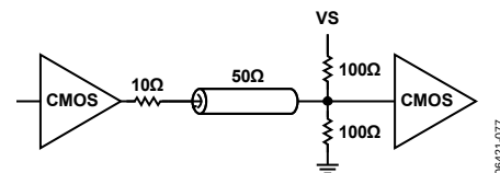
Figure 76. CMOS Output with Far-End Termination
