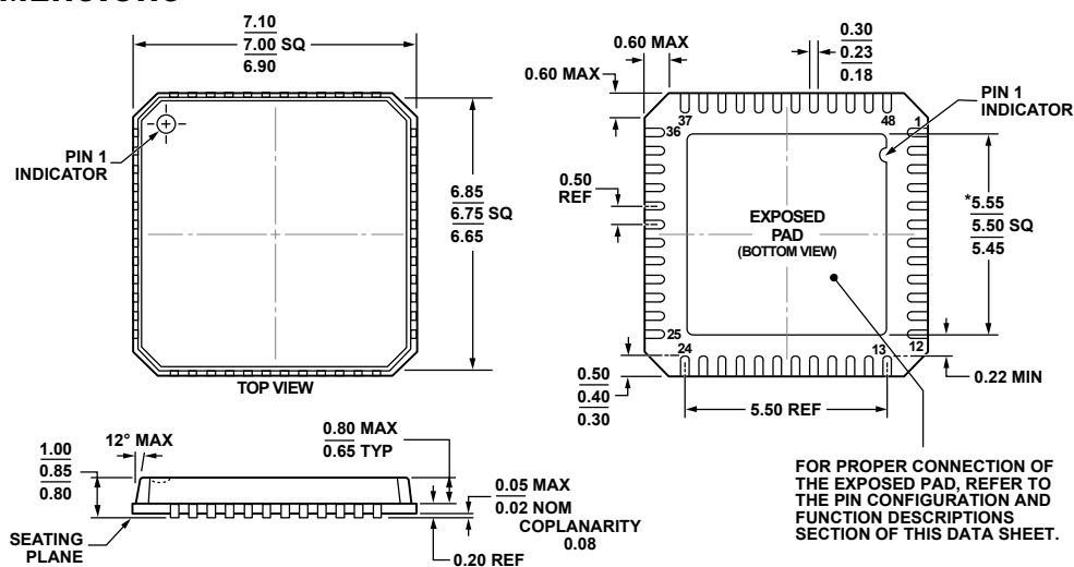
Figure 56. 48-Lead Lead Frame Chip Scale Package [LFCSP_VQ]
