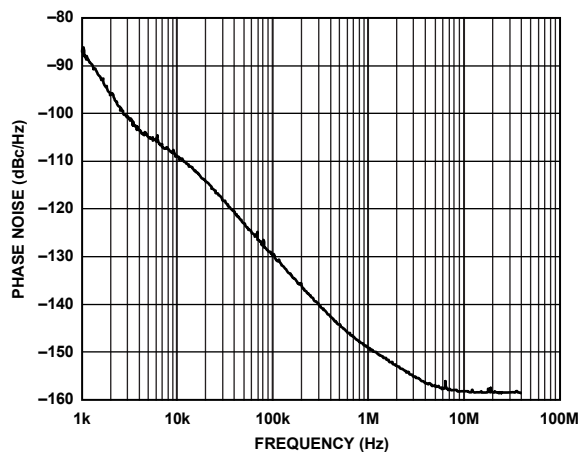
Figure 24. Phase Noise (Absolute) Clock Cleanup; Internal VCO at 2.18 GHz; PFD = 19.44 MHz; LBW = 12.8 kHz; LVPECL Output = 155.52 MHz
