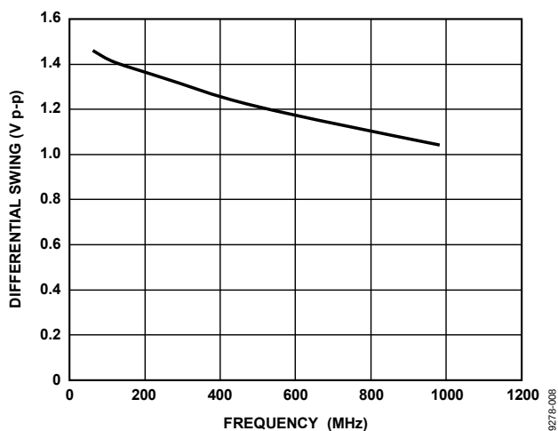
Figure 8. Differential Voltage Swing vs. Frequency, LVPECL Mode
