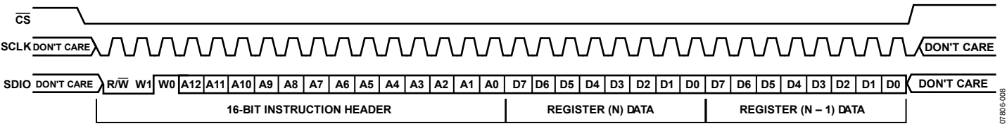
Figure 24. Serial Control Port Write—MSB First, 16-Bit Instruction, Two Bytes Data
