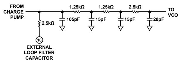
Figure 20. Internal Loop Filter
