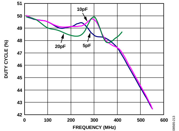
Figure 19. Duty Cycle vs. Output Frequency, CMOS
