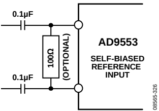
Figure 26. Reference Input
