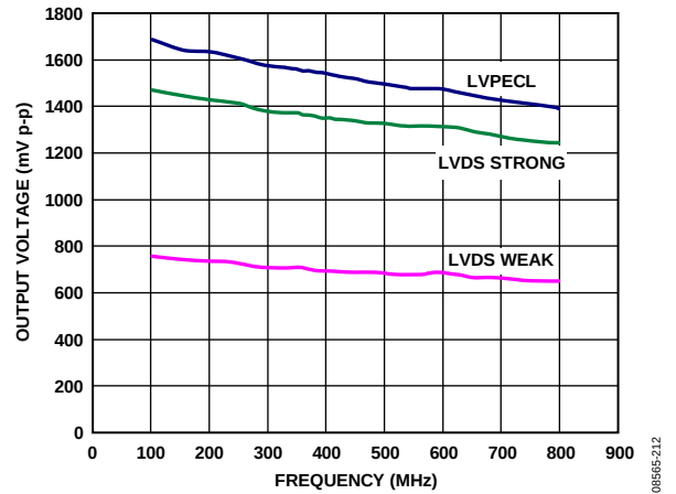
Figure 18. Peak-to-Peak Output Voltage vs. Frequency, LVPECL and LVDS (100 \Omega Load)
