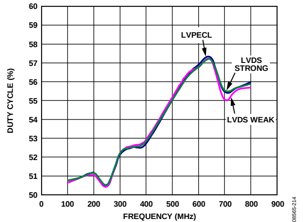
Figure 20. Duty Cycle vs. Output Frequency, LVPECL and LVDS (100 \Omega Load)
