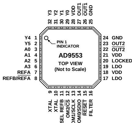
Figure 2. Pin Configuration
