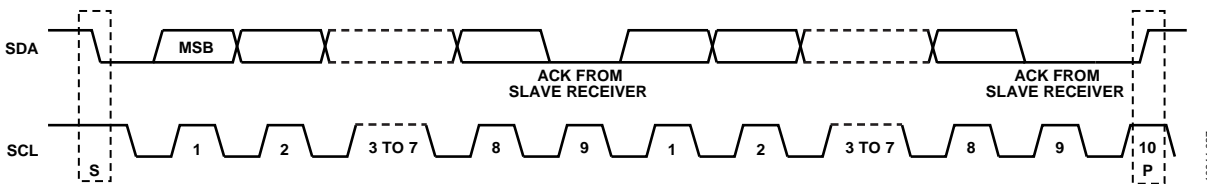
Figure 53. Acknowledge Bit
