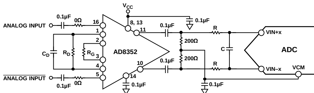
Figure 47. Differential Input Configuration Using the AD8352
