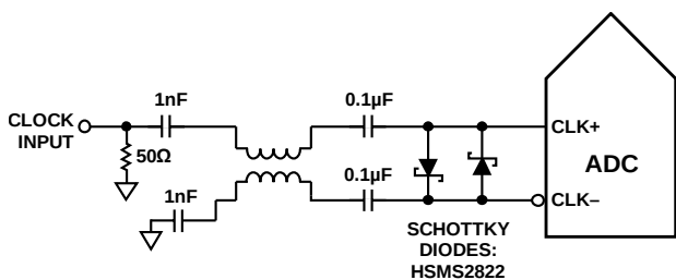
Figure 54. Balun-Coupled Differential Clock (Up to 1 GHz)
