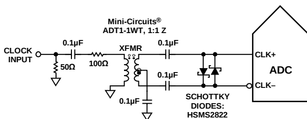
Figure 53. Transformer-Coupled Differential Clock (Up to 200 MHz)
