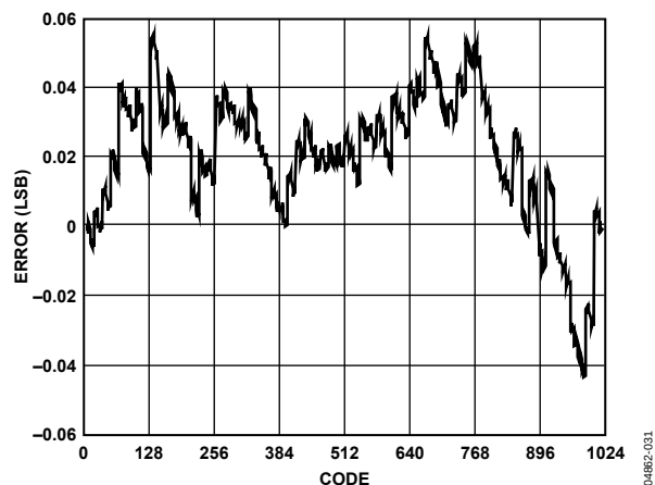
Figure 33. AD9734 INL, 25°C, 10 mA FS
