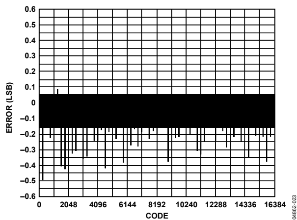
Figure 25. AD9736 DNL, 25°C, 30 mA FS
