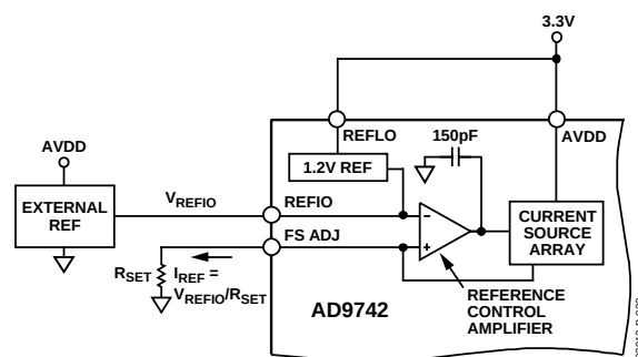
Figure 24. External Reference Configuration
