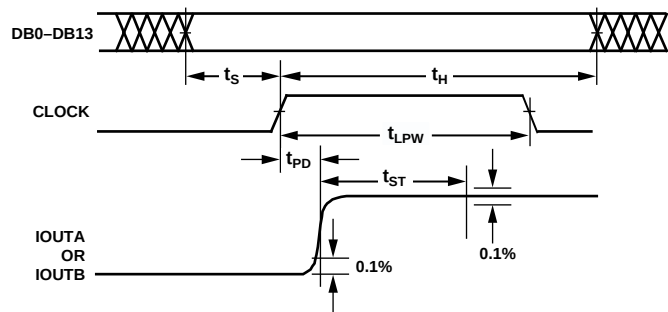
Figure 2. Timing Diagram
