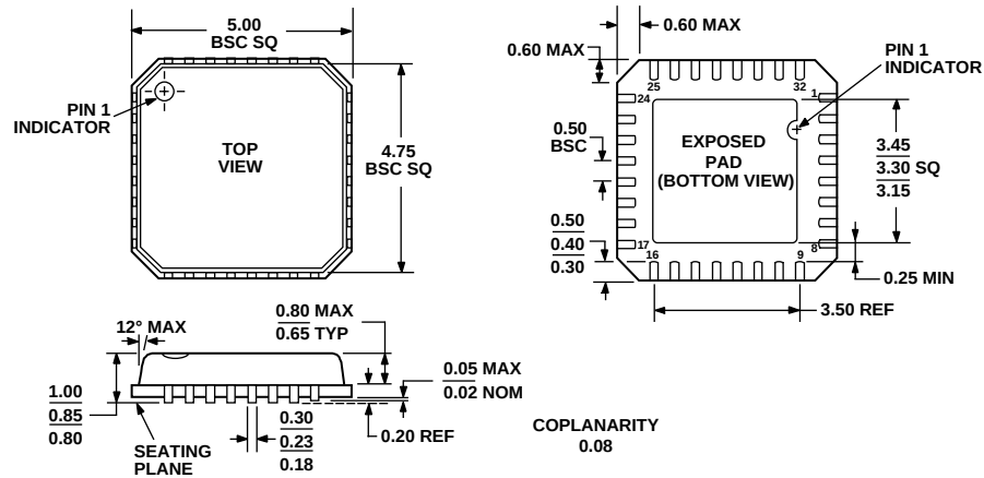
COMPLIANT TO JEDEC STANDARDS MO-220-VHHD-2 Figure 60. 32-Lead Lead Frame Chip Scale Package [LFCSP] 5 mm x 5 mm Body (CP-32-3) Dimensions shown in millimeters
