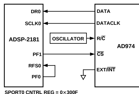
Figure 26. AD974-to-ADSP-2181 Interface
