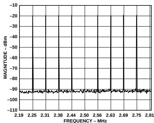
Figure 34a. Multitone Spectral Plot
