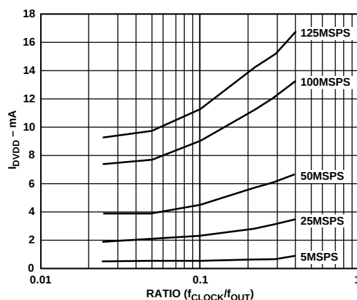
Figure 25. I_{DVDD} vs. Ratio @ DVDD = 5 \text{ V}
