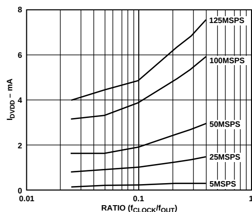
Figure 26. I_{DVDD} vs. Ratio @ DVDD = 3 \text{ V}
