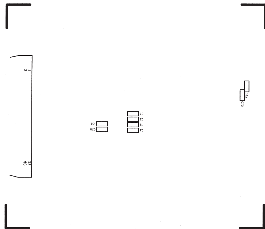
Figure 30. Silkscreen Layer—Bottom
