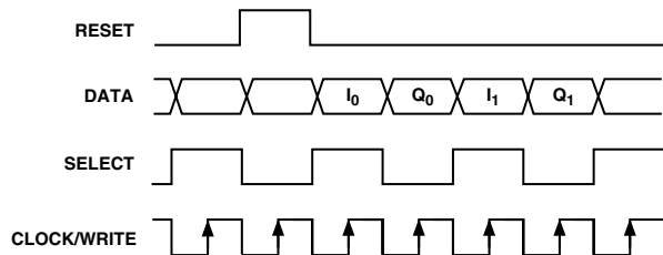
Figure 12. Timing Diagram
