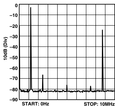
TPC 10. Single-Tone SFDR (DC to 2 f_{\text{DATA}} , f_{\text{CLOCK}} = 2 f_{\text{DATA}} )
