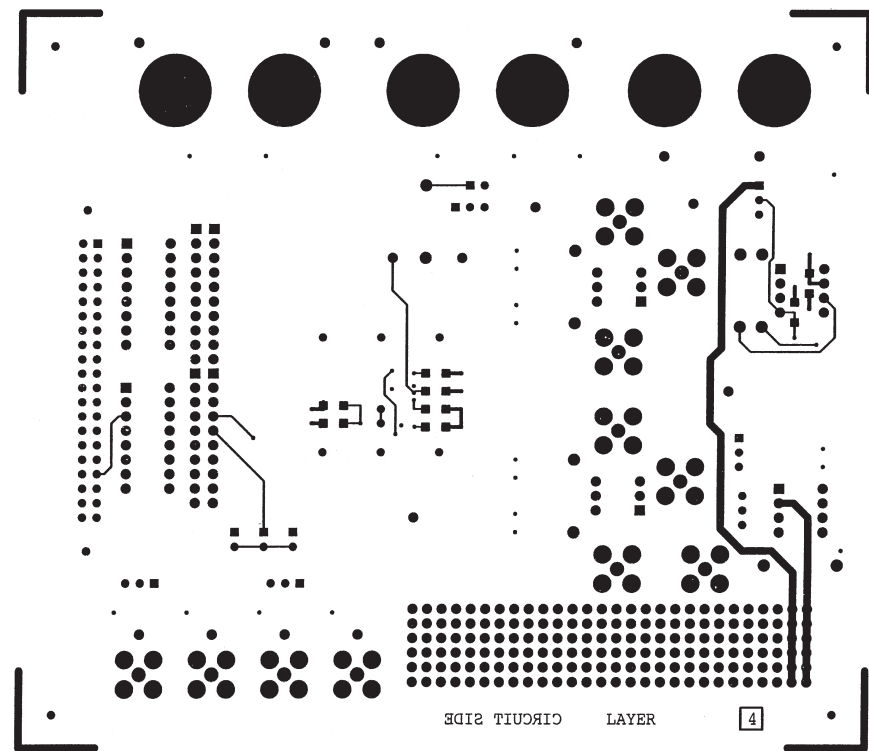
Figure 29. Solder Side PCB Layout (Layer 4)
