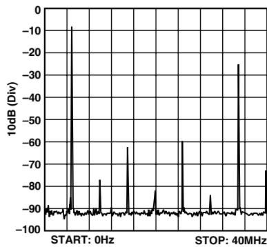
TPC 1. Single-Tone SFDR (DC to 2 f_{\text{DATA}} , f_{\text{CLOCK}} = 2 f_{\text{DATA}} )
