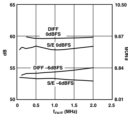
TPC 11. SINAD (ENOBs) vs. f_{\text{OUT}} (DC to f_{\text{DATA}}/2 )
