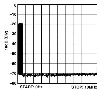
TPC 18. Narrow-Band Spread-Spectrum Spectral Plot (DC to f_{\text{DATA}} )
