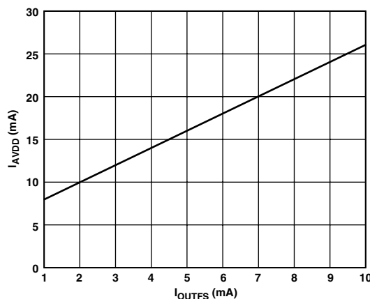
Figure 14. I_{AVDD} vs. I_{OUTFS}
