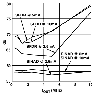
TPC 17. SINAD/SFDR vs. I_{\text{OUTFS}} (DC to f_{\text{DATA}}/2 , Single-Ended Output)
