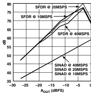
TPC 14. SINAD vs. A_{\text{OUT}} (DC to f_{\text{DATA}}/2 , Differential Output)
