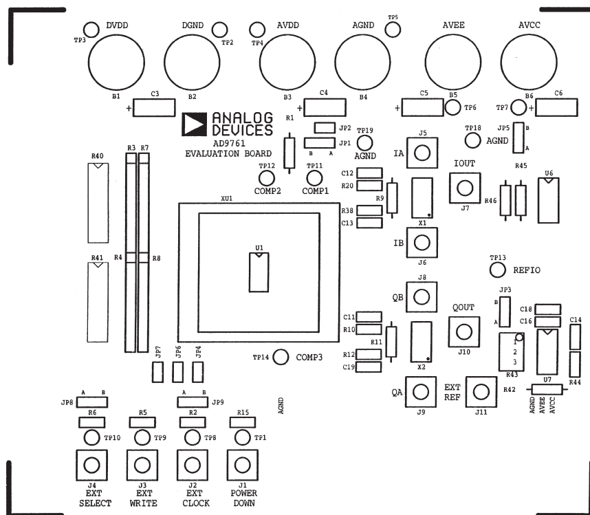
Figure 25. Silkscreen Layer—Top
