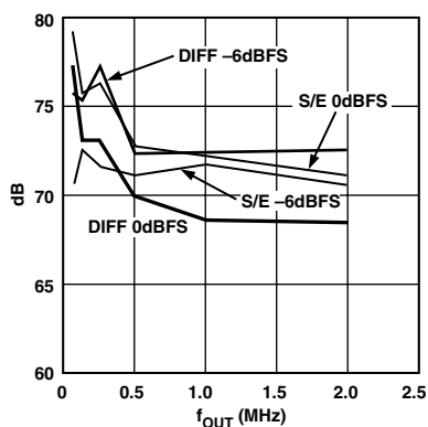
TPC 13. Out-of-Band SFDR vs. f_{\text{OUT}} ( f_{\text{DATA}}/2 to 3/2 f_{\text{DATA}} )
