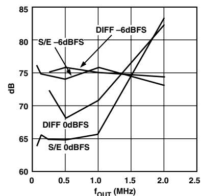
TPC 12. SFDR vs. f_{\text{OUT}} (DC to f_{\text{DATA}}/2 )
