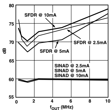
TPC 16. SINAD/SFDR vs. I_{\text{OUTFS}} (DC to f_{\text{DATA}}/2 , Differential Output)
