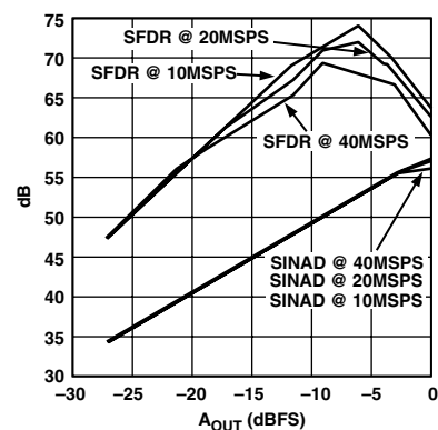
TPC 15. SINAD vs. A_{\text{OUT}} (DC to f_{\text{DATA}}/2 , Single-Ended Output)
