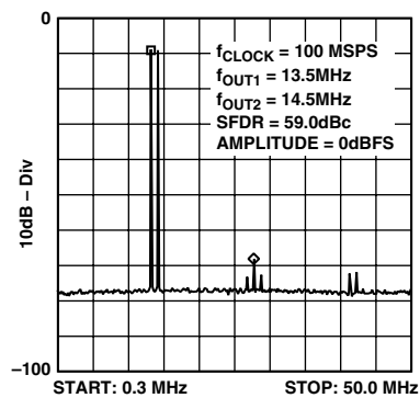
Figure 37. Dual-Tone SFDR
