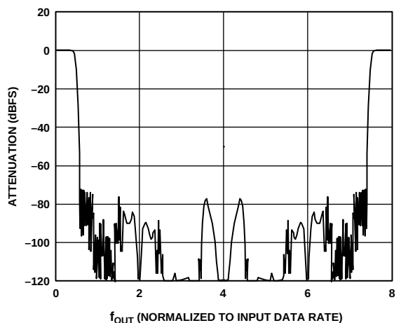
Figure 4. 8x Interpolating Filter Response
