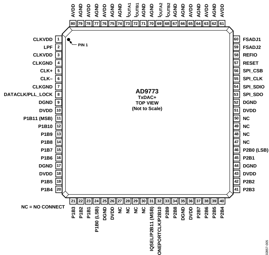
Figure 5. Pin Configuration
