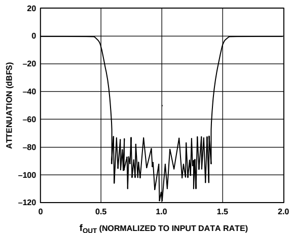
Figure 2. 2x Interpolating Filter Response
