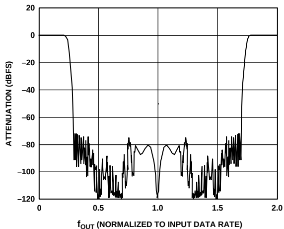
Figure 3. 4x Interpolating Filter Response
