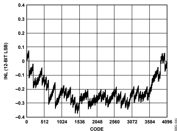
Figure 44. AD9776 Typical INL
