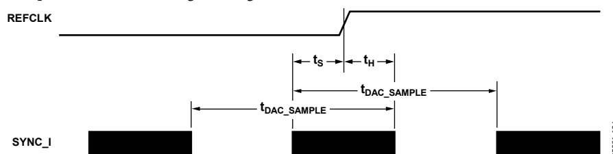
Figure 96. Valid Timing Relationship for SYNC_I to REFCLK
