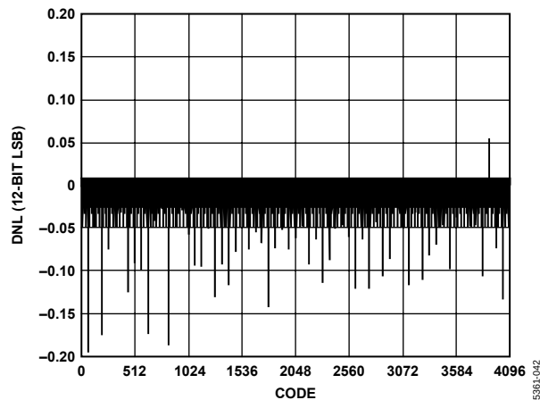
Figure 45. AD9776 Typical DNL
