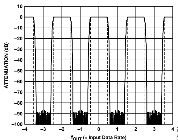
Figure 57. 2\times Interpolation, Low-Pass Response to \pm 4\times Input Data Rate (Dotted Lines Indicate 1 dB Roll-Off)
