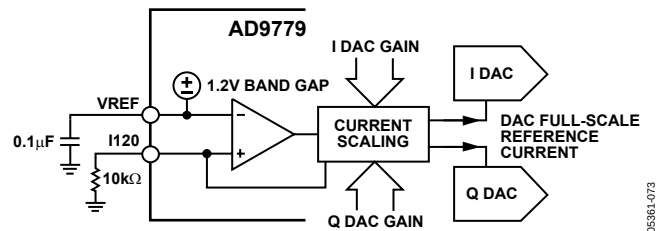
Figure 77. Reference Circuitry
