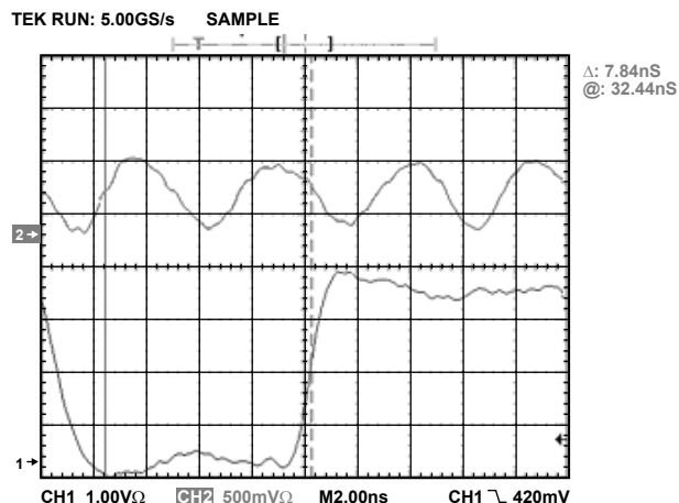
Figure 99. Delay from REFCLK to DATACLK Out with DATACLK Delay = 1111
