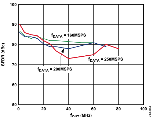
Figure 47. AD9776 In-Band SFDR, 2x Interpolation
