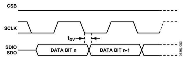
Figure 56. Timing Diagram for SPI Register Read
