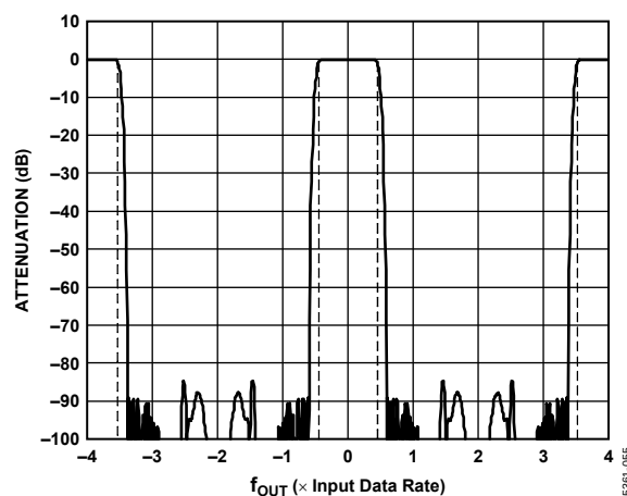
Figure 58. 4\times Interpolation, Low-Pass Response to \pm 4\times Input Data Rate (Dotted Lines Indicate 1 dB Roll-Off)
