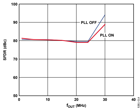
Figure 15. AD9779 In-Band SFDR, 4x Interpolation, f_{DATA} = 100 \text{ MSPS} , PLL On/Off
