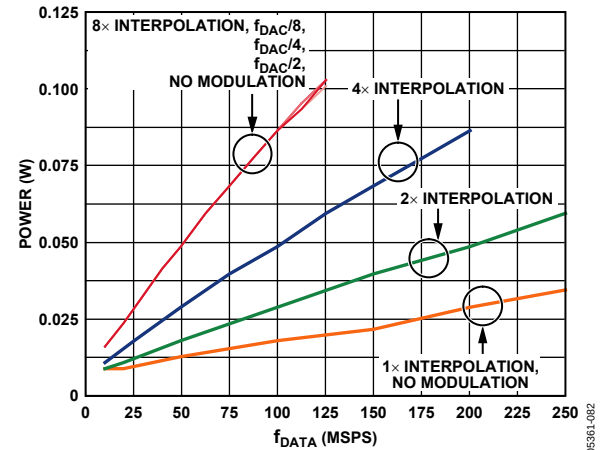
Figure 87. Power Dissipation, Clock 1.8 V Supply, I and Q Data, Dual DAC Mode, Does Not Include Zero Stuffing
