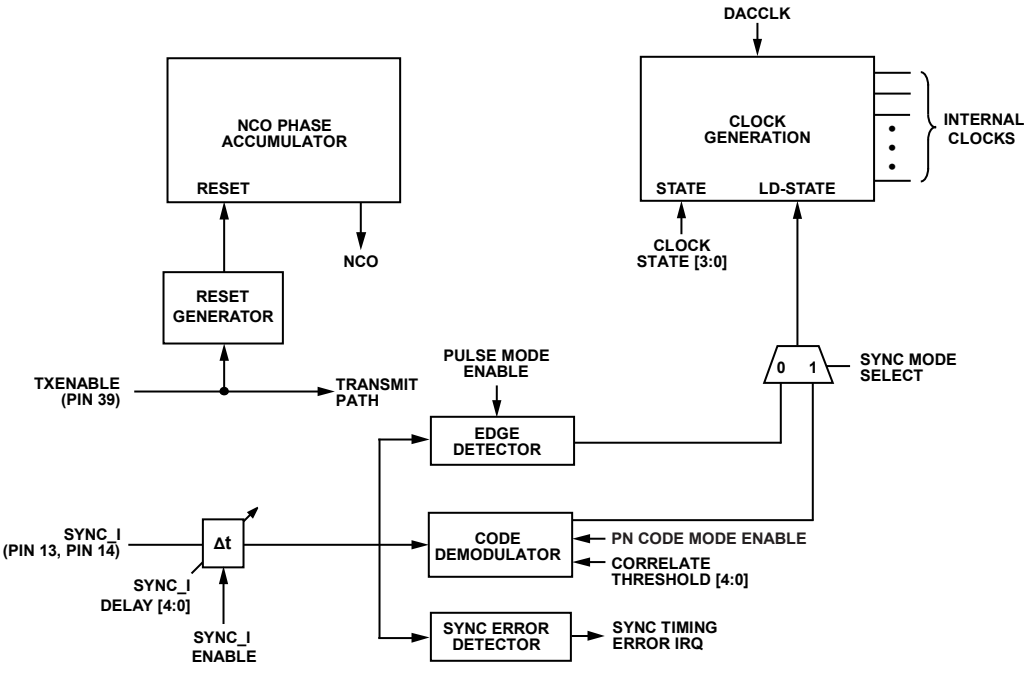
Figure 60. Synchronization Receive Circuitry Block Diagram
