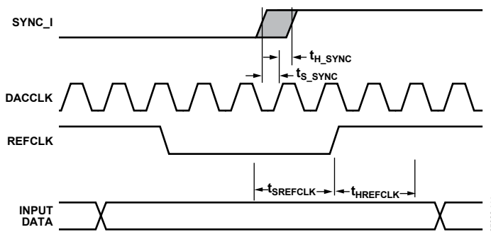
Figure 51. REFCLK 8x
