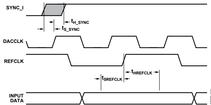
Figure 49. REFCLK 2x
