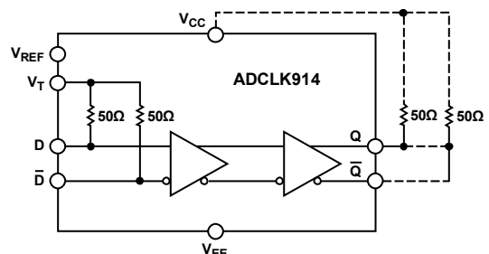
Figure 113. ADCLK914 Functional Block Diagram
