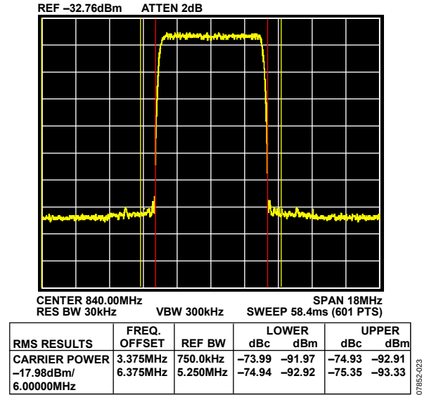
Figure 40. 1-Channel QAM ACLR, f_{OUT} = 840 MHz, Temperature = 25°C, Sum Scale = 48, Full-Scale Current = 20 mA, Span = 18 MHz
