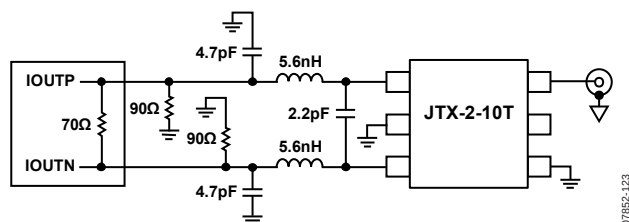
Figure 112. Recommended Transformer Output Stage for CMTS Measurements
