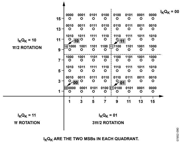
Figure 125. DVB-C 256-QAM Constellation
