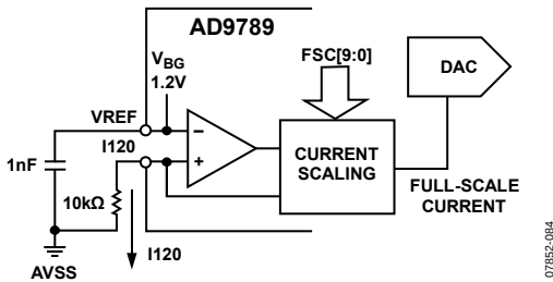
Figure 108. Voltage Reference Circuit
