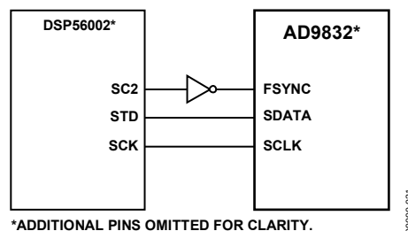
Figure 31. AD9832 to DSP56002 Interface
