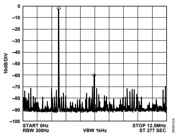
Figure 16. f_{CLK} = 25 MHz, f_{OUT} = 3.1 MHz, Frequency Word = 0x1FBE76C9
