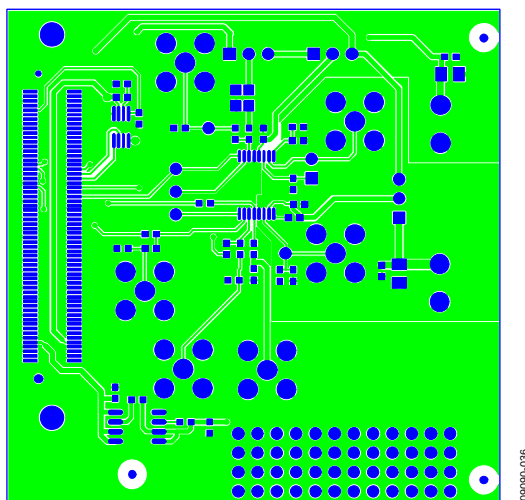
Figure 36. AD9832 Evaluation Board Component Side
