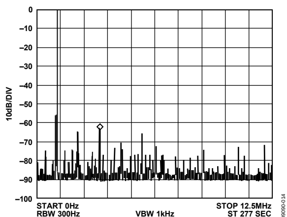
Figure 14. f_{CLK} = 25 MHz, f_{OUT} = 1.1 MHz, Frequency Word = 0xB439581
