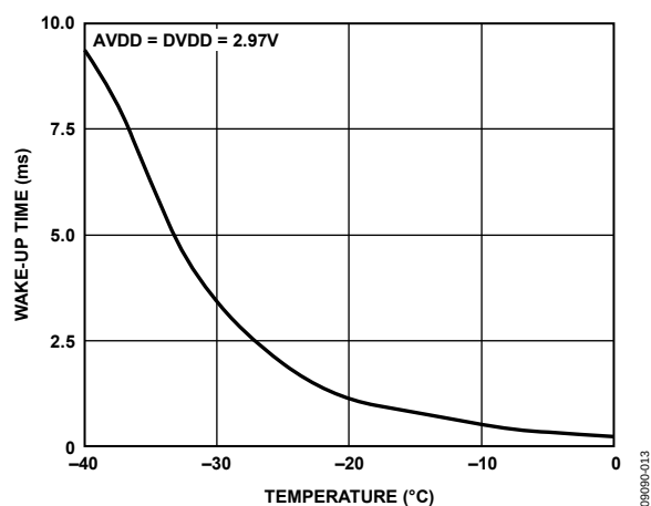
Figure 13. Wake-Up Time vs. Temperature
