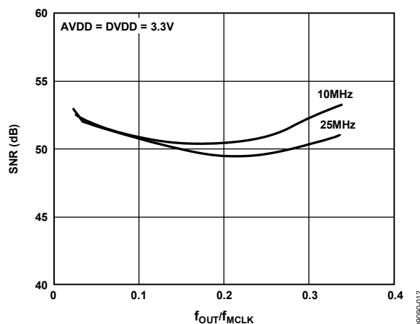
Figure 12. SNR vs. f_{OUT}/f_{MCLK} for Various MCLK Frequencies
