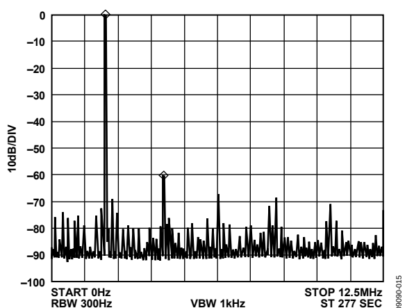
Figure 15. f_{CLK} = 25 MHz, f_{OUT} = 2.1 MHz, Frequency Word = 0x15810625
