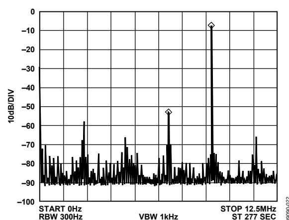
Figure 22. f_{MCLK} = 25 \text{ MHz} , f_{OUT} = 9.1 \text{ MHz} , Frequency Word = 0x5D2F1AA0
