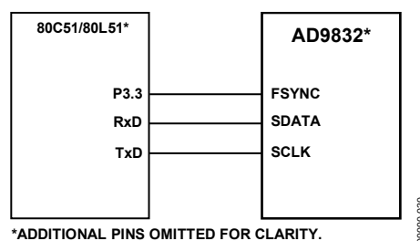
Figure 30. 80C51/80L51 to AD9832 Interface
