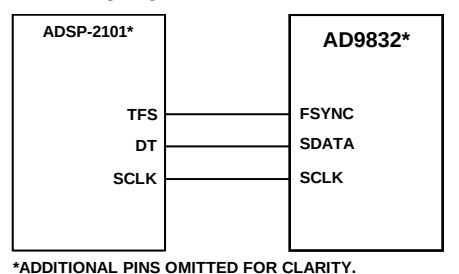
Figure 28. ADSP-2101 to AD9832 Interface
