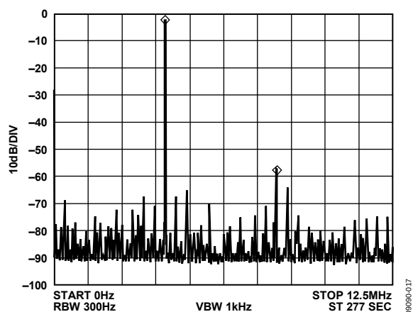
Figure 17. f_{CLK} = 25 MHz, f_{OUT} = 4.1 MHz, Frequency Word = 0x29FBE76D
