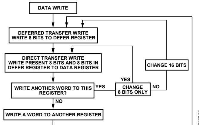
Figure 26. Data Writes
