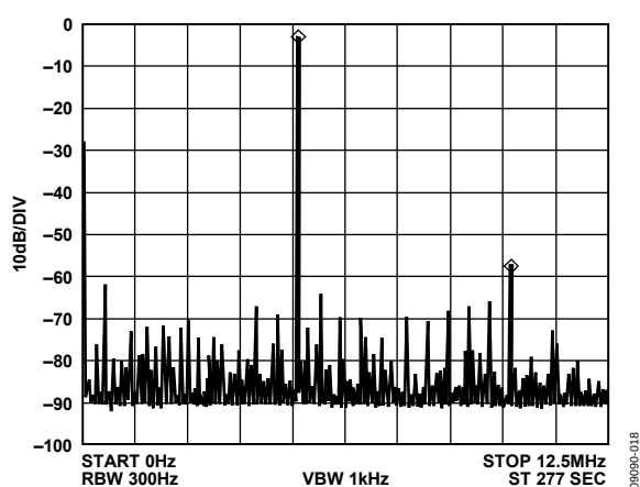
Figure 18. f_{CLK} = 25 MHz, f_{OUT} = 5.1 MHz, Frequency Word = 0x34395810
