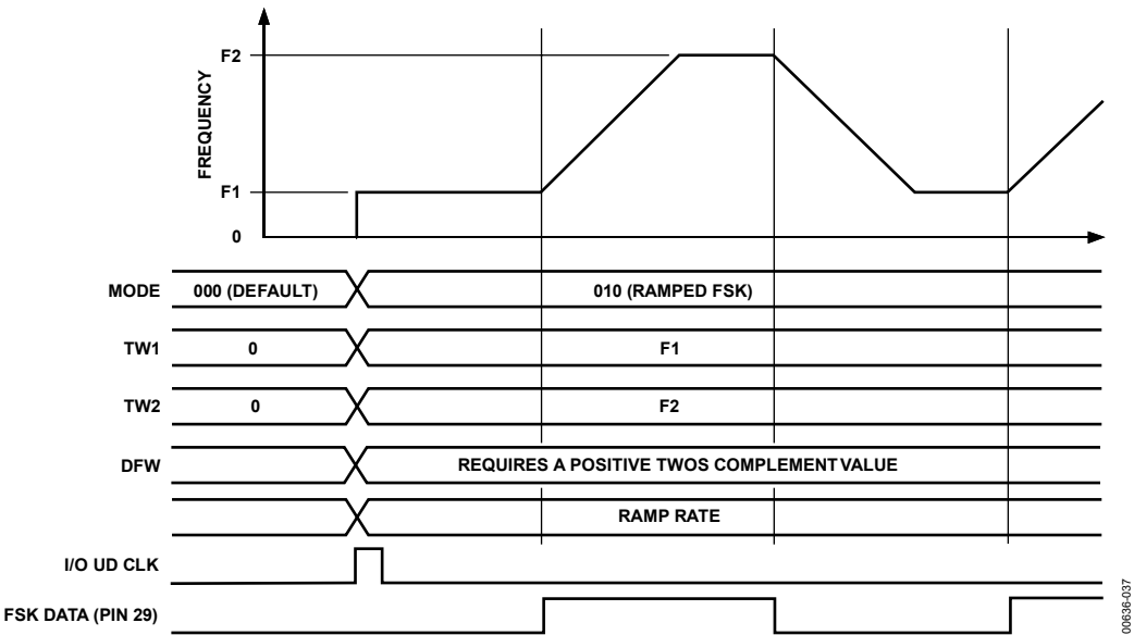
Figure 37. Ramped FSK Mode (Start at F1)
