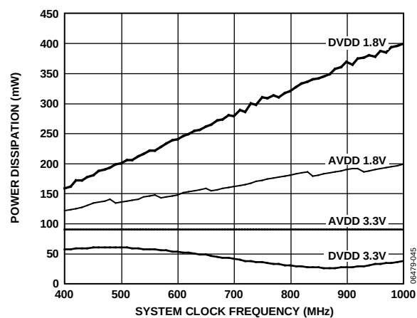
Figure 18. Power Dissipation vs. System Clock Frequency (PLL Enabled)
