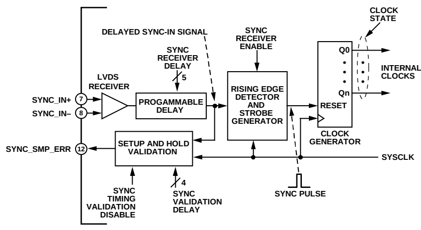
Figure 52. Sync Receiver Diagram
