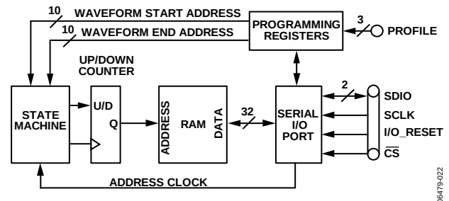
Figure 41. RAM Data Load/Retrieve Operation
