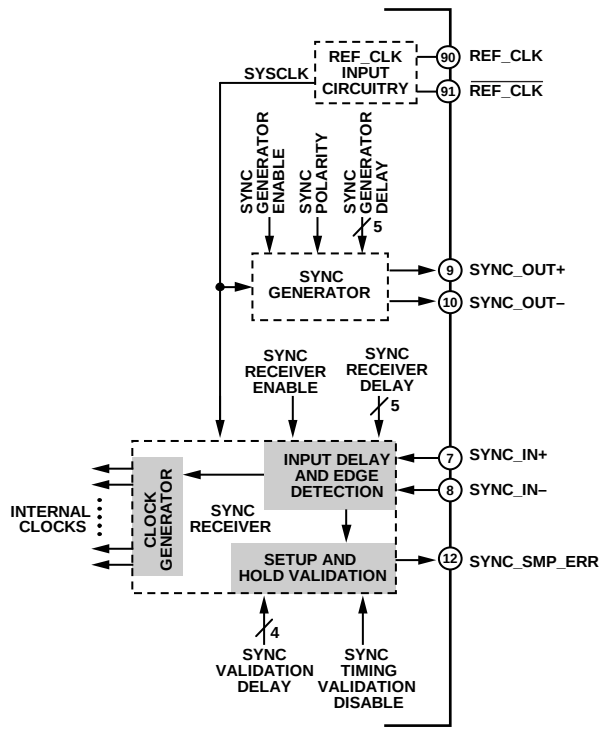
Figure 50. Synchronization Circuit Block Diagram
