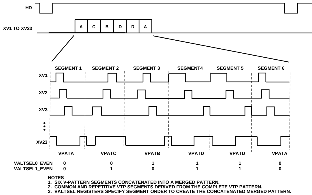
Figure 49. Example of Special V-Sequence Alternation Mode Using VALTSEL Registers to Specify Segment Order
