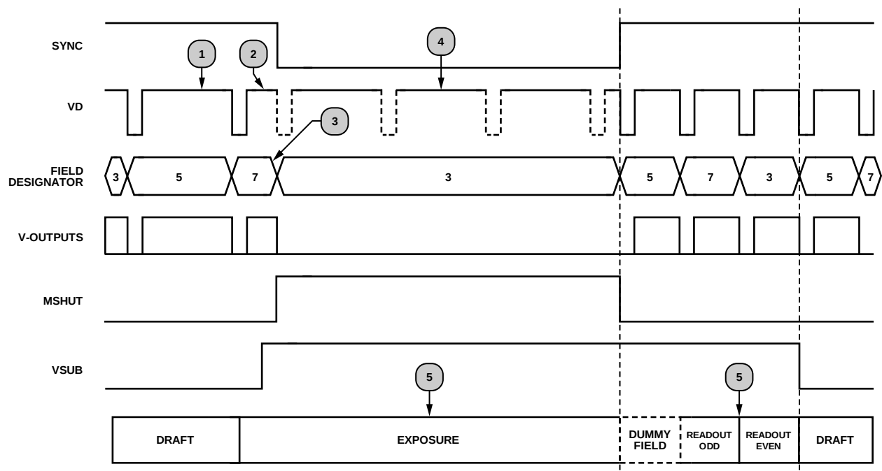
SHUTTER OPERATION IN SLR MODE 1REFER TO STEP 1. 2REFER TO STEP 2. 3REFER TO STEP 3. 4REFER TO STEP 4. 5SUBCK OUTPUT IS SUPPRESSED DURING EXPOSURE AND READOUT WHEN EXPOSURE TRIGGER IS USED.
