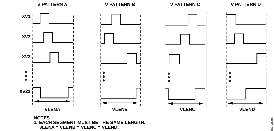
Figure 47. Vertical Timing Divided into Four Segments: VPATA, VPATB, VPATC, and VPATD
