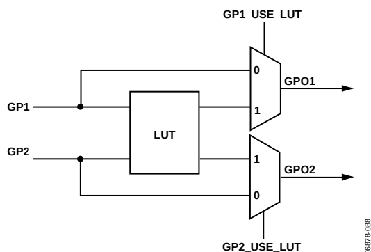
Figure 88. Internal LUT for GPO1 and GPO2 Signals
