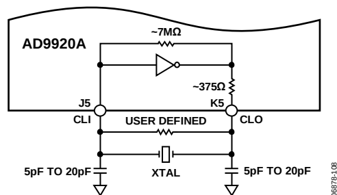
Figure 108. Crystal Application Using CLI/CLO
