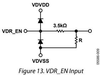
Figure 13. VDR_EN Input
