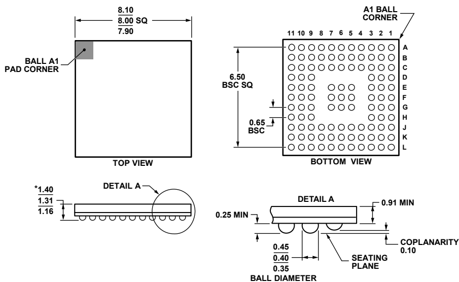
*COMPLIANT TO JEDEC STANDARDS MQ-225 WITH THE EXCEPTION TO PACKAGE HEIGHT. Figure 89. 105-Lead Chip Scale Package Ball Grid Array [CSP_BGA] (BC-105) Dimensions shown in millimeters
