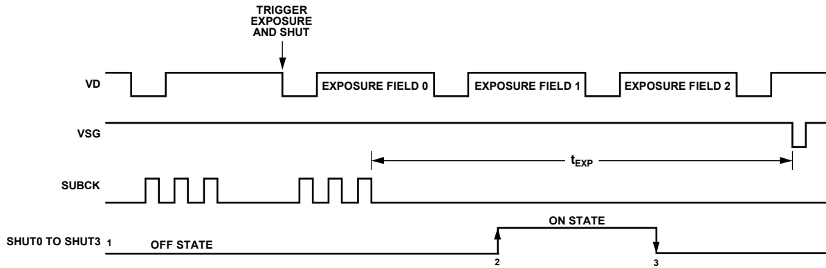
Figure 70. Single Trigger Control of SHUT0 to SHUT3 Signals
