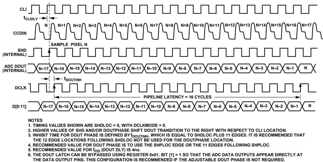
Figure 22. Digital Data Output Pipeline Delay
