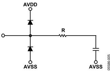
Figure 9. CCDIN, CCDGND
