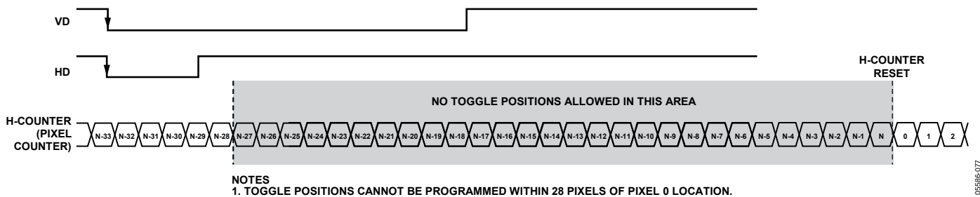
Figure 79. Toggle Position Inhibited Area—Slave Mode
