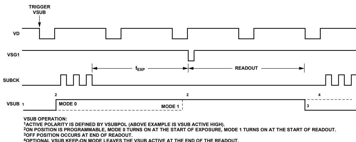
Figure 67. VSUB0, VSUB1 Signal Programmability
