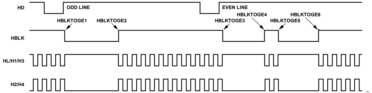
ALTERNATING H-BLANK PATTERN USING HBLKALT = 1 MODE. Figure 29. HBLK Odd/Even Alternation Using HBLKALT = 1
