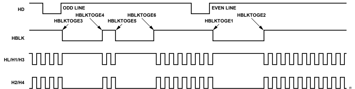
ALTERNATING H-BLANK PATTERN USING HBLKALT = 2 MODE. Figure 30. HBLK Odd/Even Alternation Using HBLKALT = 2
