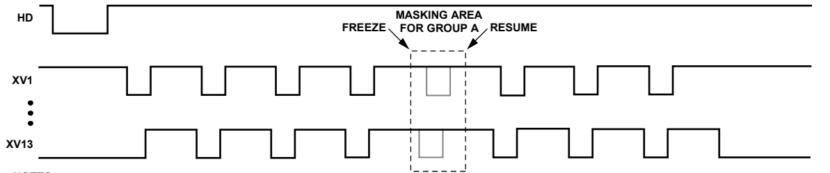
Figure 43. Using FREEZE/RESUME
