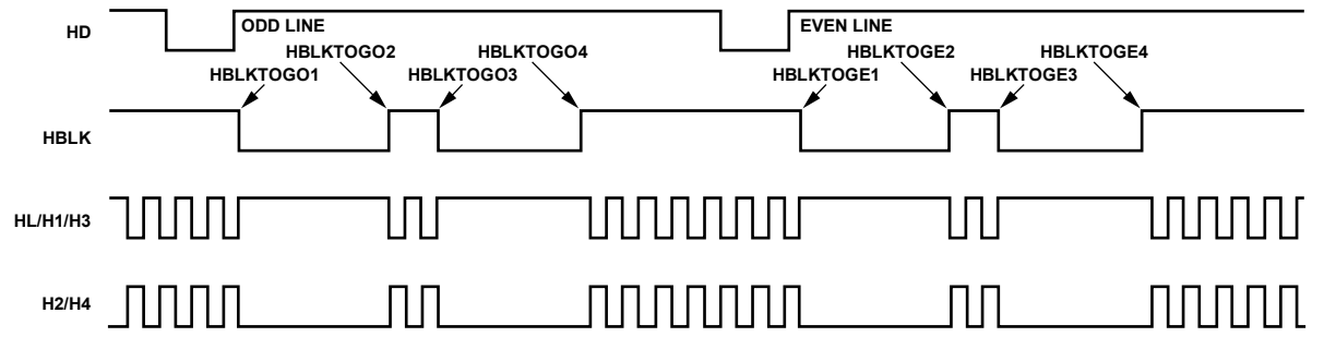
ALTERNATING H-BLANK PATTERN USING HBLKALT = 3 MODE. (FREEZE/RESUME FUNCTION NOT AVAILABLE IN THIS MODE.) Figure 31. HBLK Odd/Even Alternation Using HBLKALT = 3
