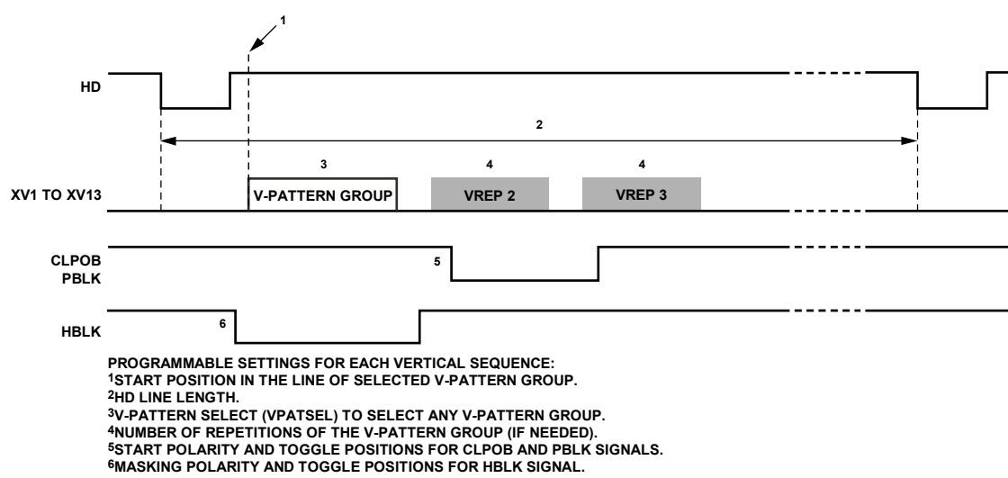
Figure 37. V-Sequence Programmability
