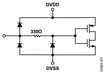
Figure 11. Digital Inputs
