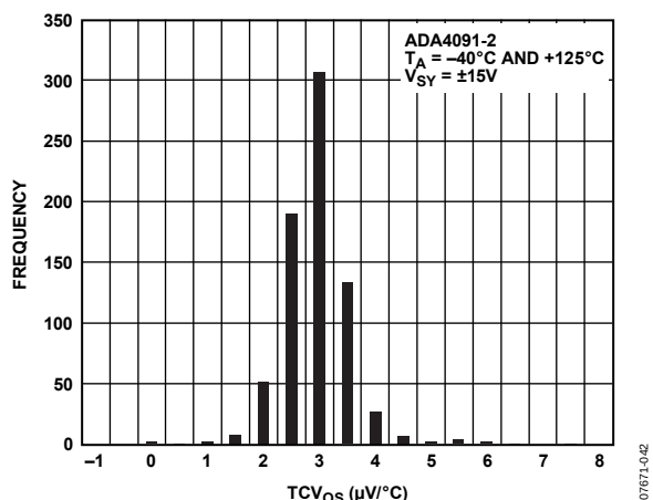
Figure 27. Offset Voltage TC
