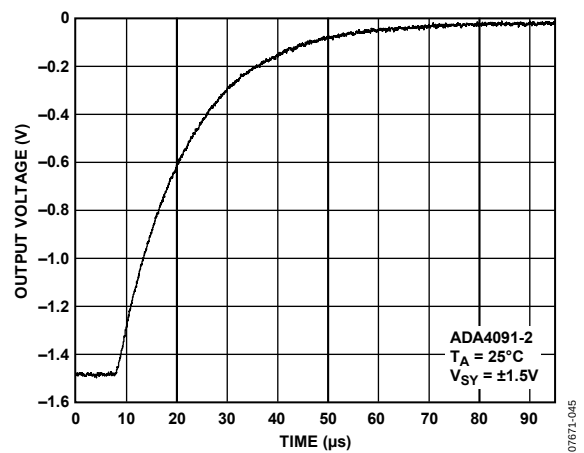
Figure 13. Negative Overload Recovery
