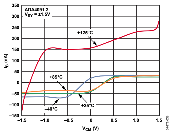
Figure 4. Input Bias Current vs. Input Common-Mode Voltage
