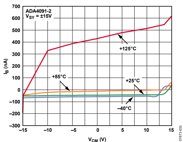
Figure 28. Input Bias Current vs. Common-Mode Voltage
