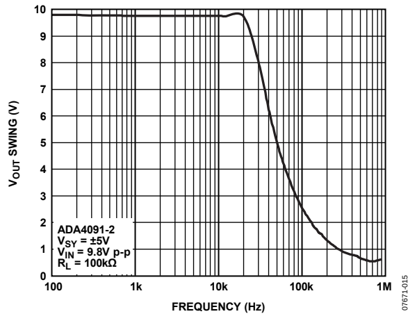
Figure 21. Output Voltage Swing vs. Frequency
