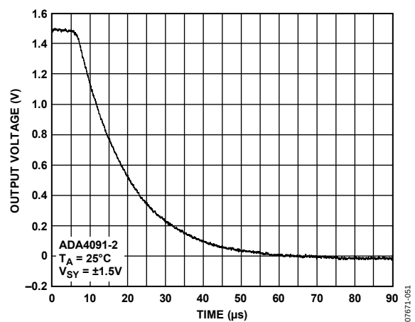
Figure 12. Positive Overload Recovery
