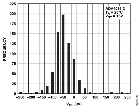
Figure 14. Input Offset Voltage Distribution
