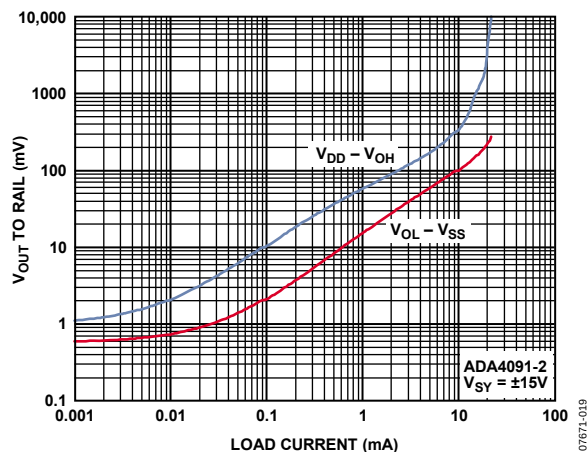
Figure 33. Dropout Voltage vs. Load Current
