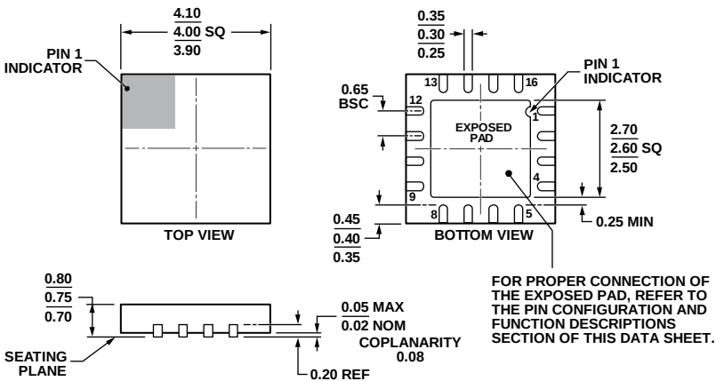
Figure 53. 16-Lead Lead Frame Chip Scale Package [LFCSP_WQ] 4 mm x 4 mm Body, Very Very Thin Quad (CP-16-17) Dimensions are millimeters
