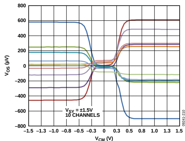
Figure 10. Input Offset Voltage ( V_{OS} ) vs. Common-Mode Voltage ( V_{CM} )
