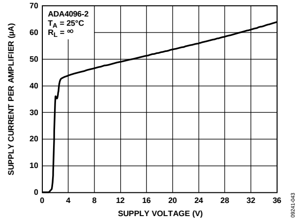
Figure 50. Supply Current per Amplifier vs. Supply Voltage
