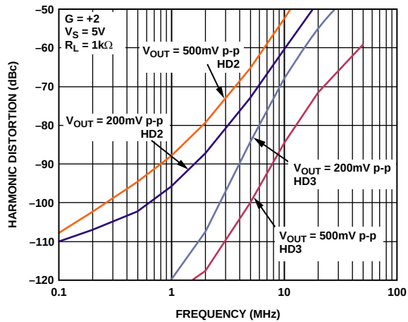
Figure 18. Harmonic Distortion vs. Frequency for Various V_{OUT}
