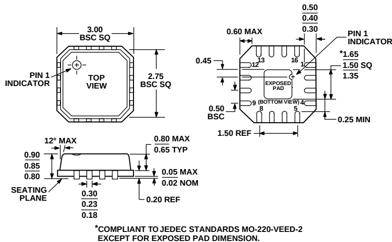
*COMPLIANT TO JEDEC STANDARDS MO-220-VEED-2 EXCEPT FOR EXPOSED PAD DIMENSION. Figure 42. 16-Lead Lead Frame Chip Scale Package [LFCSP_VQ] 3 mm × 3 mm Body, Very Thin Quad (CP-16-3) Dimensions shown in millimeters
