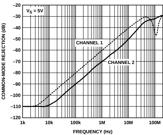
Figure 37. Common-Mode Rejection Ratio (CMRR) vs. Frequency
