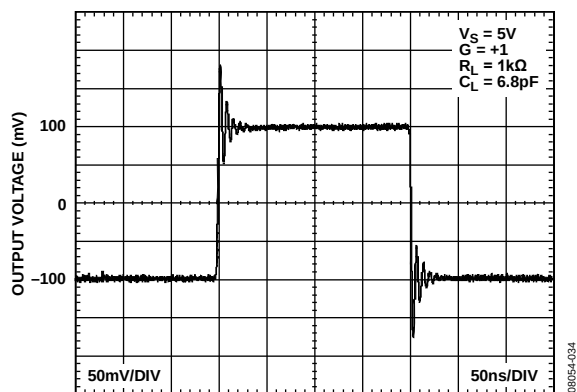
Figure 56. 200 mV Step Response, C_L = 6.8\text{ pF} , ADA4891-1/ADA4891-2
