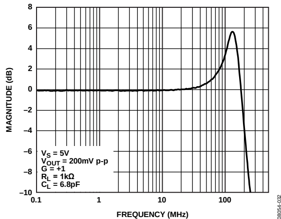
Figure 55. Closed-Loop Frequency Response, C_L = 6.8\text{ pF} , ADA4891-1/ADA4891-2
