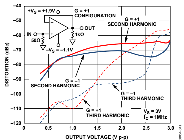
Figure 24. Harmonic Distortion (HD2, HD3) vs. Output Voltage, V_S = 3\text{ V}
