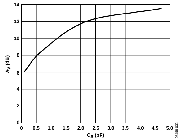
Figure 37. Recommended C_S Values for Most Gains
