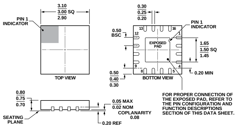
Figure 46. 16-Lead Lead Frame Chip Scale Package [LFCSP_WQ] 3 mm x 3 mm Body, Very Very Thin Quad (CP-16-27) Dimensions shown in millimeters
