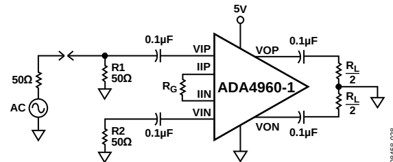
Figure 32. Single-Ended-Input-to-Differential-Output Configuration
