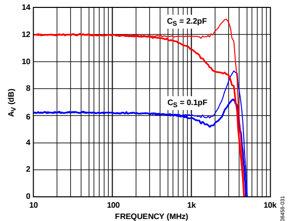
Figure 36. Bandwidth Extension for 6 dB and 12 dB Gains
