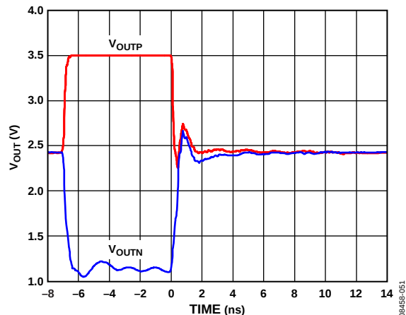
Figure 42. Output Overdrive, V_{IN} = 1 V p-p, A_V = 12 dB
