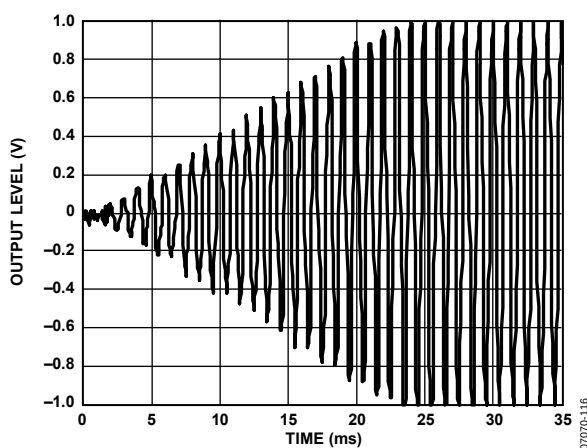
Figure 44. Slew RAM—Constant Time Update Increasing Ramp, Full Scale
