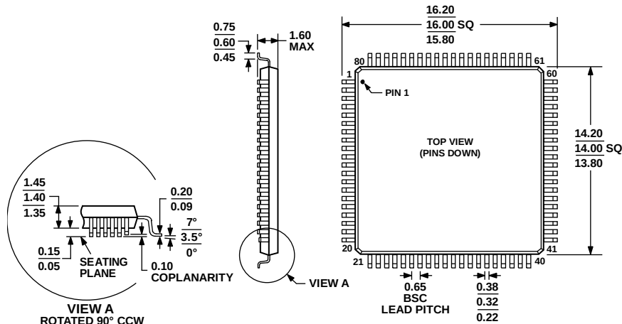
COMPLIANT TO JEDEC STANDARDS MS-026-BEC Figure 35. 80-Lead Low Profile Quad Flat Package [LQFP] (ST-80-2) Dimensions shown in millimeters
