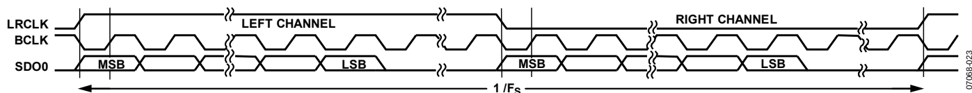
Figure 27. Left-Justified Mode
