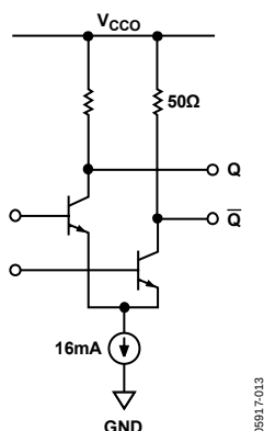
Figure 14. Simplified Schematic Diagram of CML-Compatible Output Stage
