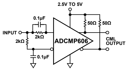
Figure 19. Self-Biased, 50% Slicer
