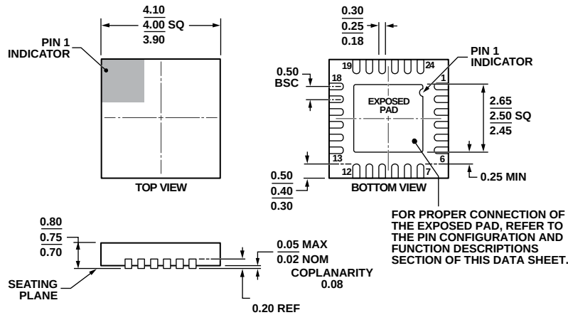
Figure 24. 24-Lead Lead Frame Chip Scale Package [LFCSP_WQ] 4 mm x 4 mm Body, Very Very Thin Quad (CP-24-7) Dimensions shown in millimeters
