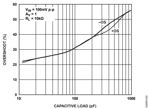
Figure 28. Channel V_{COM} Small Signal Overshoot vs. Load Capacitance
