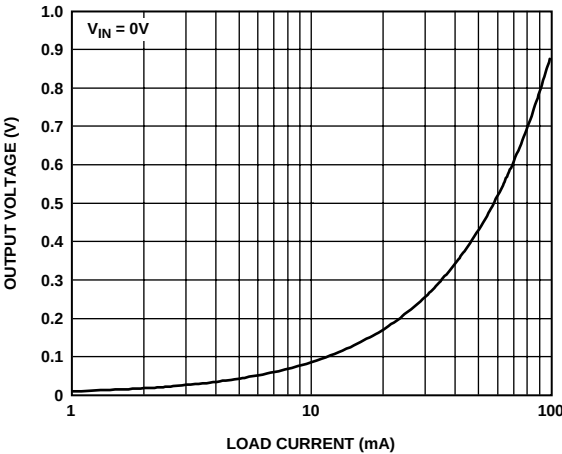
Figure 12. Channel V_{COM} Output Voltage Low vs. I Load
