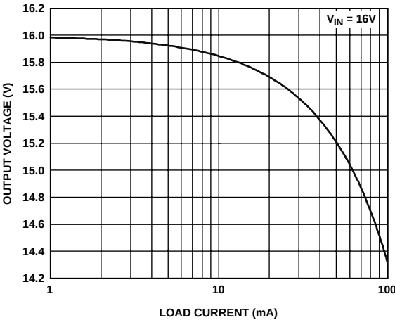
Figure 13. Channel 1 Output Voltage High vs. I Load
