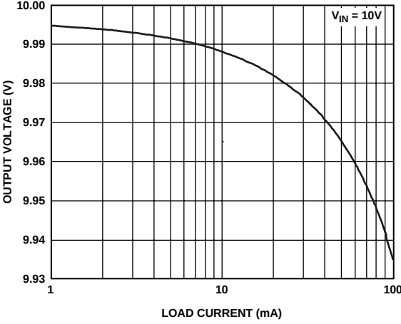
Figure 14. Channels 2 to 5 Output Voltage High vs. I Load
