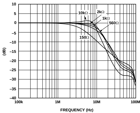
Figure 23. Channels 6 to 10 Frequency Response vs. Resistive Loading
