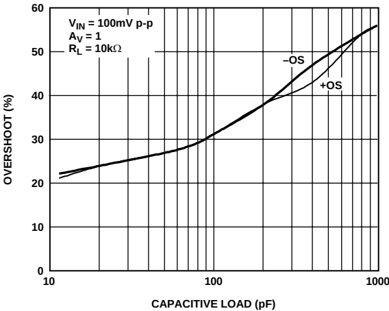
Figure 28. Channel V_{COM} Small-Signal Overshoot vs. Load Capacitance
