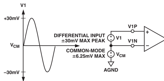
Figure 5. Maximum Signal Levels, Channel V1
