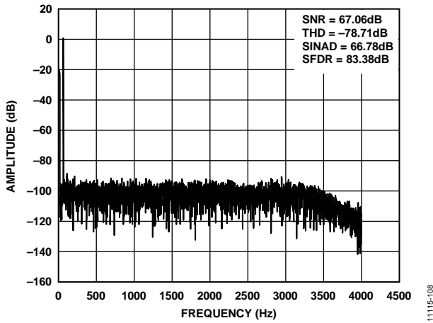
Figure 6. Current Channel Fast Fourier Transform (FFT), \pm 31.25 mV, 50 Hz Pseudo Differential Input Signal, ADC\_FREQ = 8 kHz, BW = 3300 Hz
