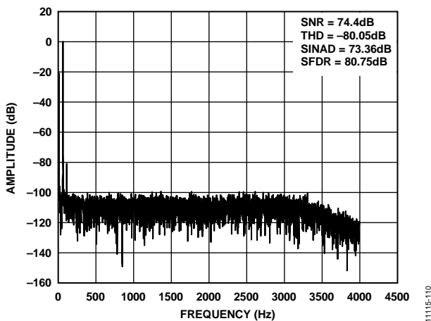
Figure 8. Voltage Channel V1 FFT, \pm 500 mV, 50 Hz Pseudo Differential Input Signal, ADC\_FREQ = 8 kHz, BW = 3300 Hz
