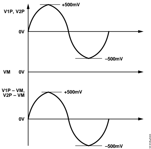
Figure 20. Pseudo Differential Input Voltage Range Between V1P and VM Pins and Between V2P and VM
