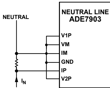
Figure 28. Neutral Line with the ADE7903
