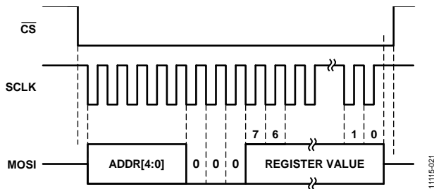
Figure 36. SPI Write Operation
