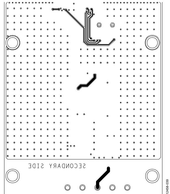
Figure 39. 2-Layer Circuit Board Bottom Layer
