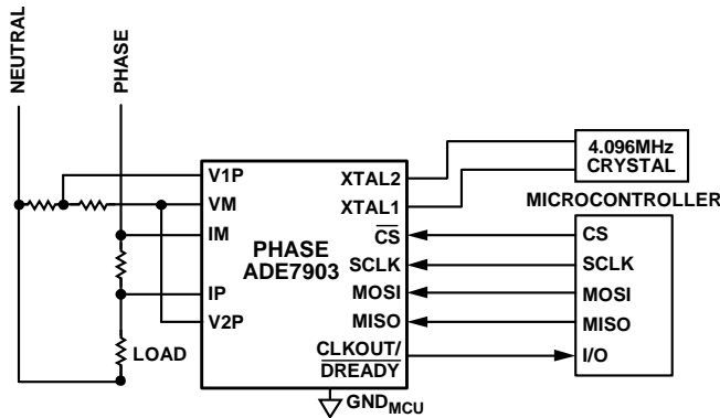
Figure 32. 1-Phase Energy Meter Using an ADE7903 Device
