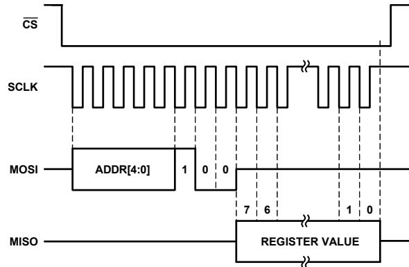
Figure 34. SPI Read Operation of an 8-Bit Register
