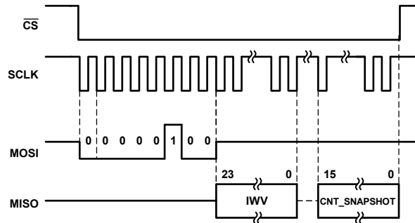
Figure 35. SPI Read Operation in Burst Mode
