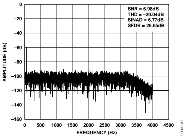
Figure 7. Current Channel FFT, \pm 31.25 \mu V, 50 Hz Pseudo Differential Input Signal, ADC\_FREQ = 8 kHz, BW = 3300 Hz
