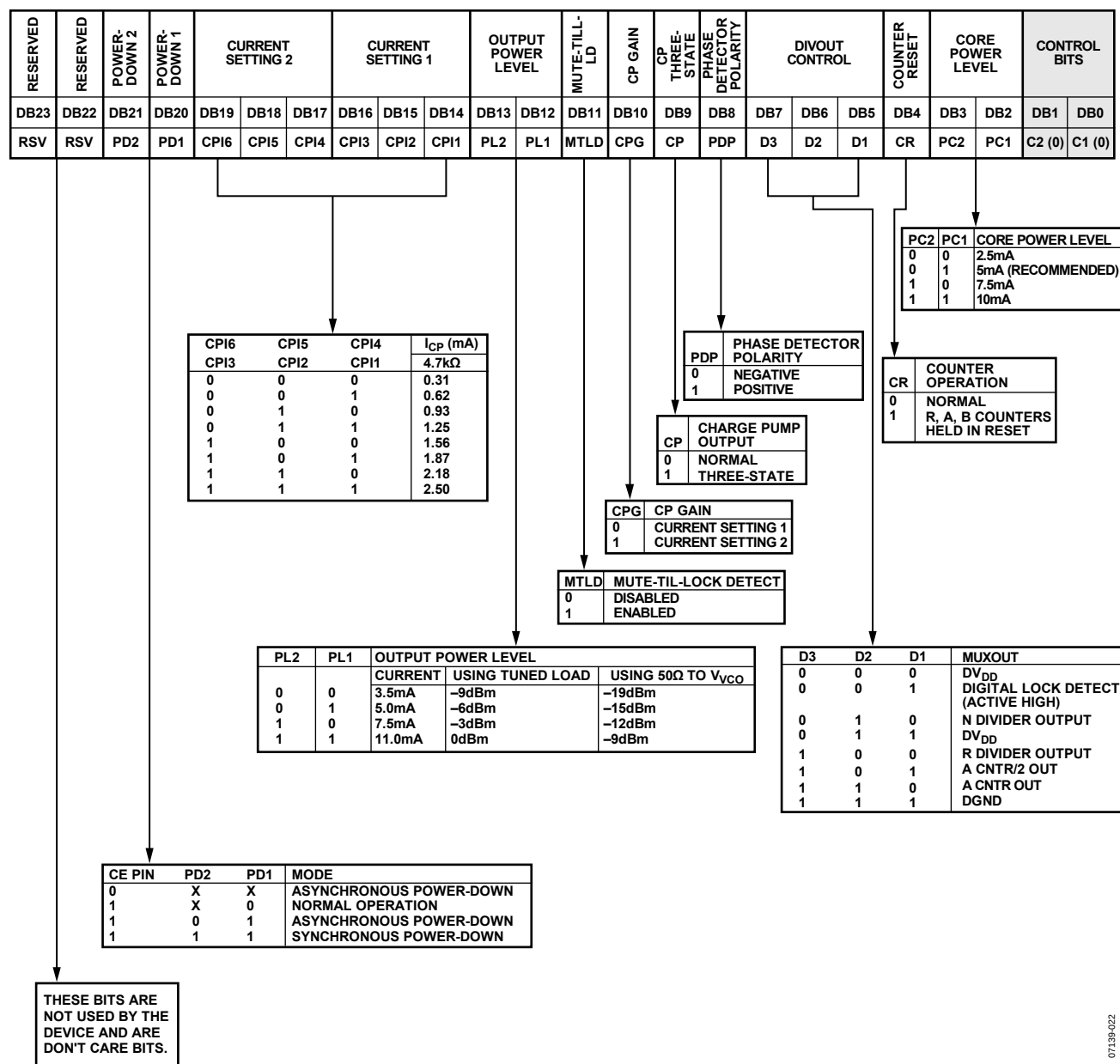
Figure 23. Control Latch
