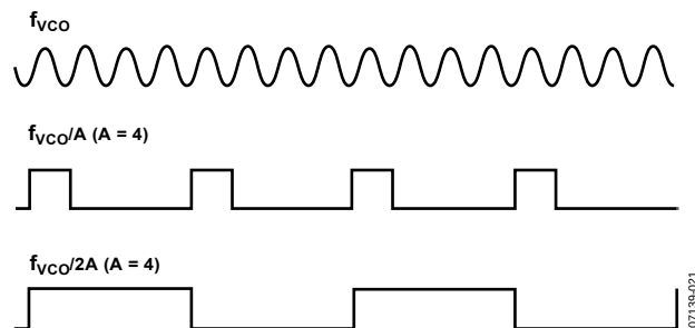
Figure 21. DIVOUT Waveforms
